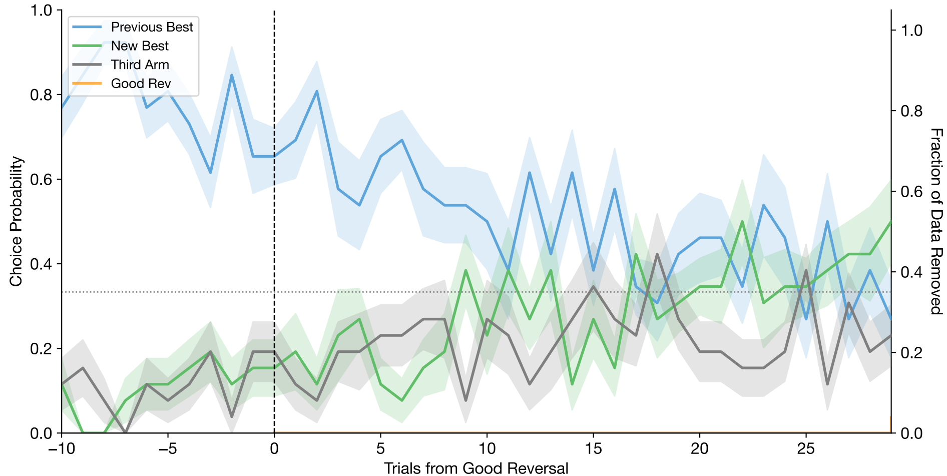
Good Reversal-Aligned Choices (mean \pm se across subjects | n=13 subjects, n=26 reversals)
